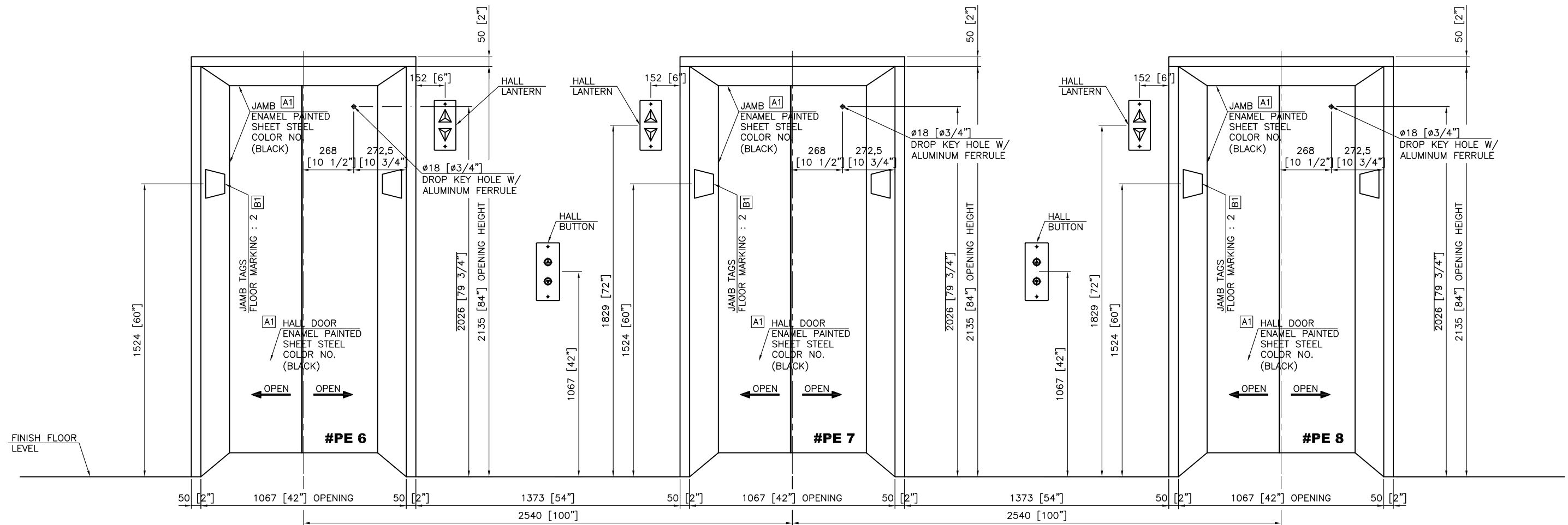
ENTRANCE ELEVATION WIDE STRAIGHT JAMB : 2 FL [B1]
