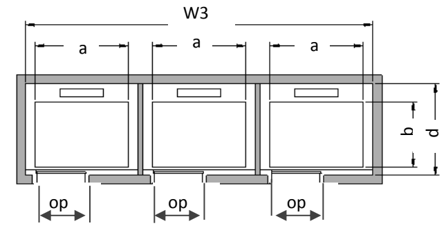
HOISTWAY PLAN
