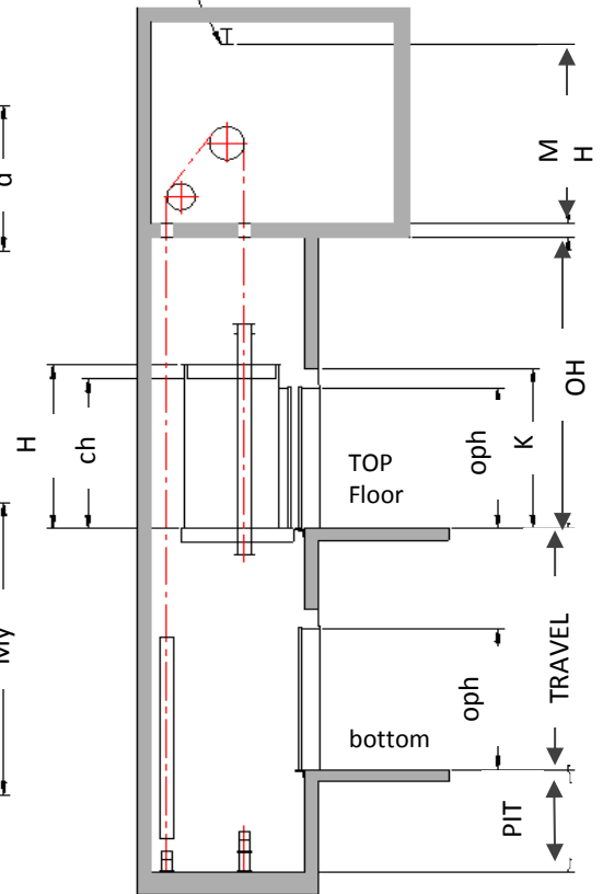
HOISTWAY SECTION
